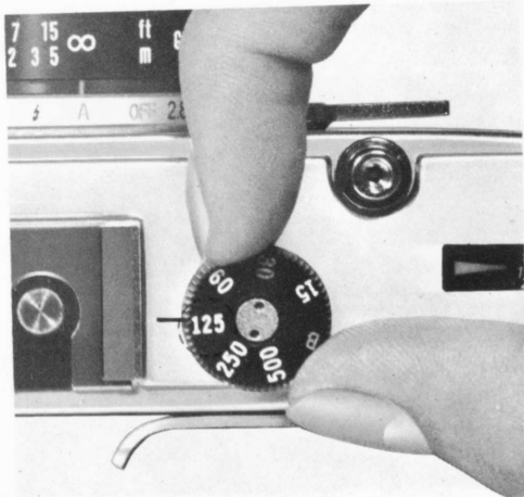
4 Set the shutter speed dial according to the subject to be photographed. (See page 17.)
