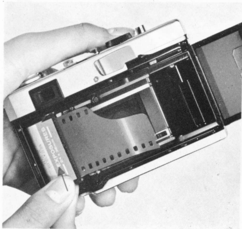
3 Insert film magazine onto rewind shaft.
