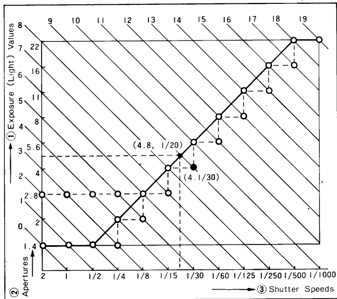
• Exposure combinations of programmed automatic exposure (ASA 100)
